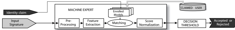
Figure 1. System model for person authentication based on handwritten signature.
