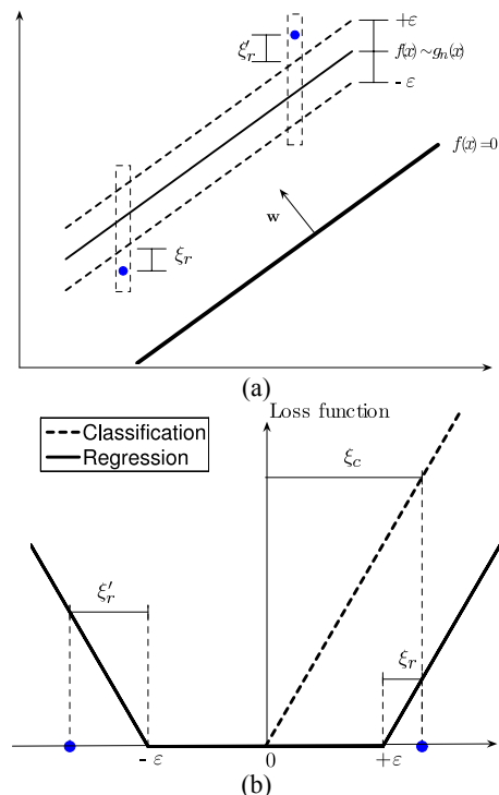
Figure 1. SVR vs. SVC. Boundaries (a) and loss functions (b).
