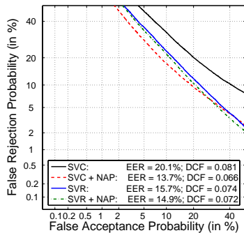
Figure 2. DET curve of SVC, SVC + NAP, SVR and SVR + NAP systems in NIST SRE 2008 short2-short3 task.
