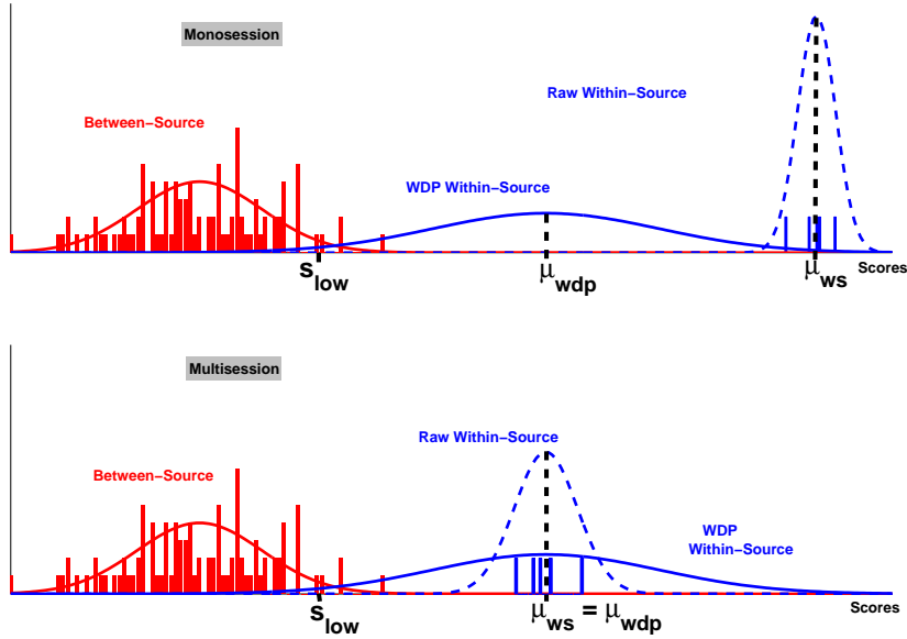
Fig. 7. Within-source Degradation Prediction (WDP).
