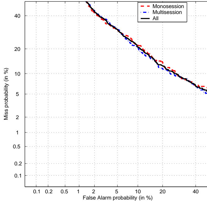
Fig. 9. ATVS NIST SRE 2002 system performance with Switchboard I data. The reference raw scores are the basis for all algorithms in section 4.
