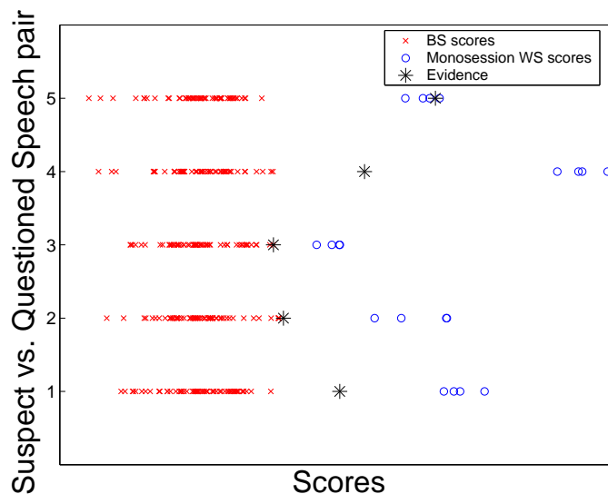
Fig. 6. Plot of between-source (BS), monosession within-source (WS) and Evidence scores in five sample cases extracted from the NIST SRE 2004 ATVS results.
