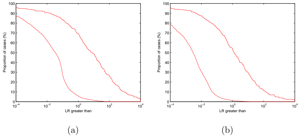
Fig. 16. NFI/TNO eval'03 “Court Proof” condition. (a) Dutch population (ATVS-2b) and (b) TDLRA (ATVS-2c).
