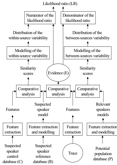
Fig. 1. LR Computation Steps.
