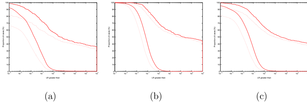
Fig. 12. Tippett plots for same system of Figure 11 adding TDLRA. Two configurations for TDLRA are shown, with maximum Non-Target errors of 1% (dotted) and 3% (solid).
