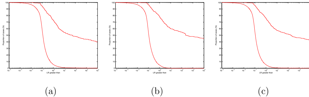
Fig. 11. Tippet Plots using WDP, WMVL and Outlier removal. (a) 'Monosession', (b) 'multisession' and (c) 'all' suspect Switchboard data.
