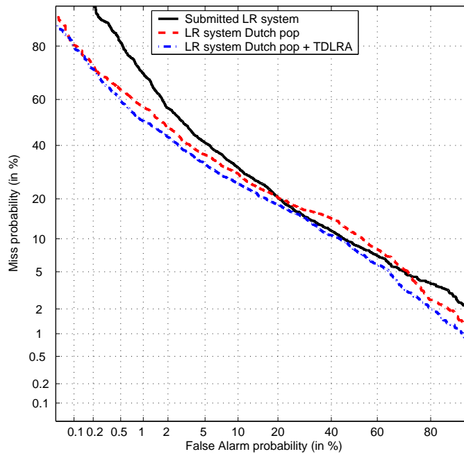
Fig. 15. ATVS forensic systems at NFI/TNO eval'03. Submitted (ATVS-2a), same system with Dutch population (ATVS-2b) and TDLRA system with Dutch pop. (ATVS-2c)
