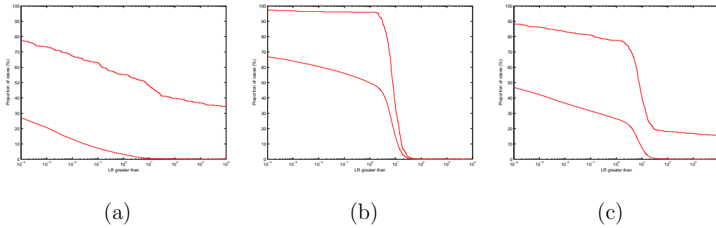
Fig. 10. Tippet Plots with Raw LR. (a) 'Monosession', (b) 'multisession' and (c) 'all' suspect Switchboard data.
