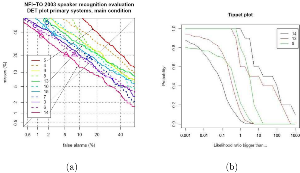
Fig. 5. (a) NFI-TNO 2003 Evaluation main task results and (b) Court Proof results. Source: [15].
