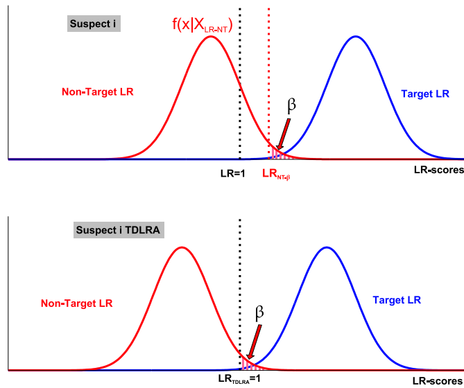
Fig. 8. Target Dependent Likelihood Ratio Alignment (TDLRA).
