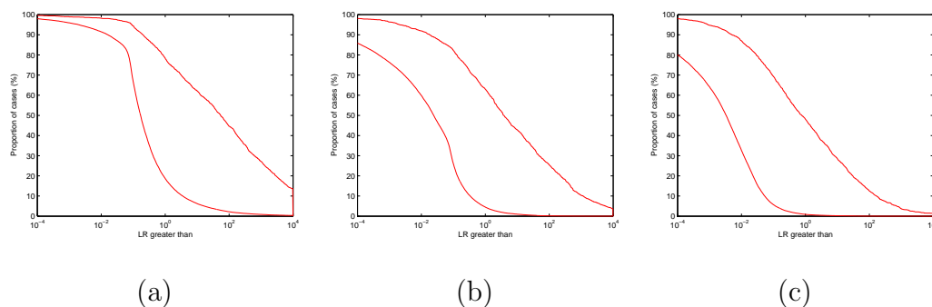
Fig. 14. ATVS forensic systems at NFI/TNO eval'03. (a) Submitted (ATVS-2a), (b) same system with Dutch reference population (ATVS-2b) and (c) TDLRA system with Dutch reference population. (ATVS-2c)
