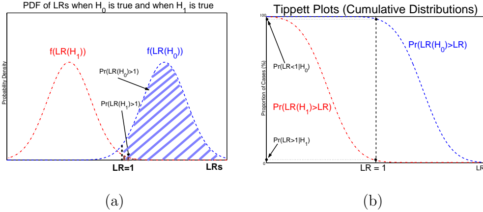
Fig. 4. (a) PDF of LR s in H_0 and H_1 hypothesis, and (b) Tippett plots (cumulative density functions of LR s matching each of the two competing hypotheses).
