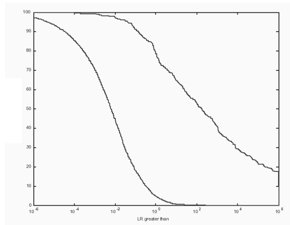
Fig. 17. Tippet plot of the ATVS LR system obtained from warping+TNorm scores in the NFI Eval primary condition (Post-Evaluation experiments).
